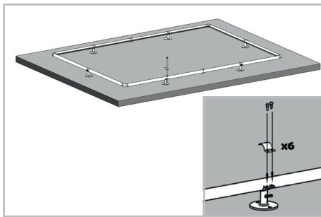
Mounting the wall brackets
