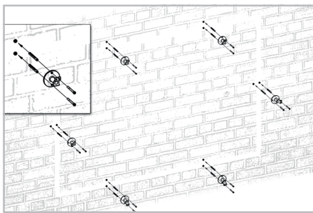
Fixation of the wall brackets
